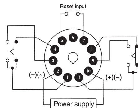
With Reset Input (H3CR-H8L)
